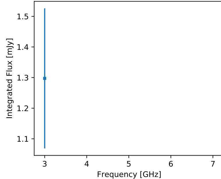
F357 J171904.17-342605.9 (unr)
