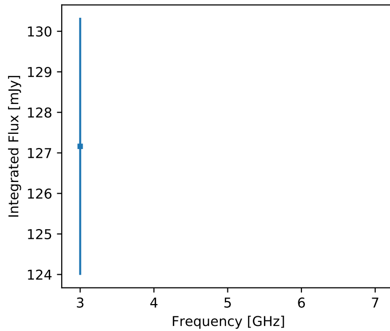
F357 J171640.95-321411.3 (unr)
