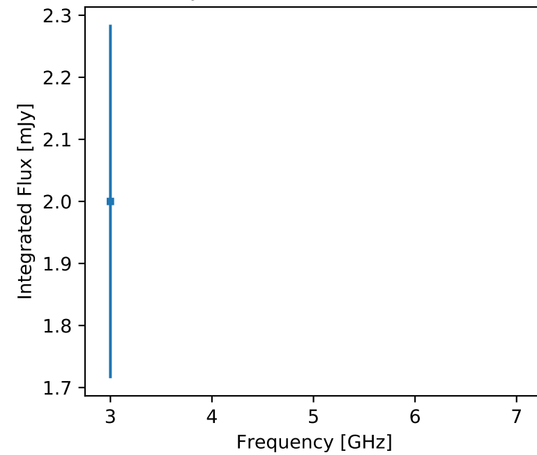
F357 J171707.66-321521.5 (unr)
