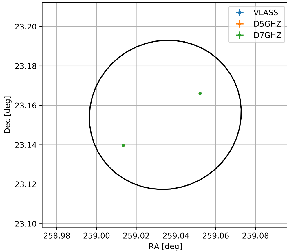
4FGL J1716.1+2309
