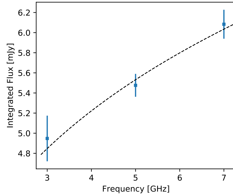
F357 J171612.51+230957.9 (unr)
