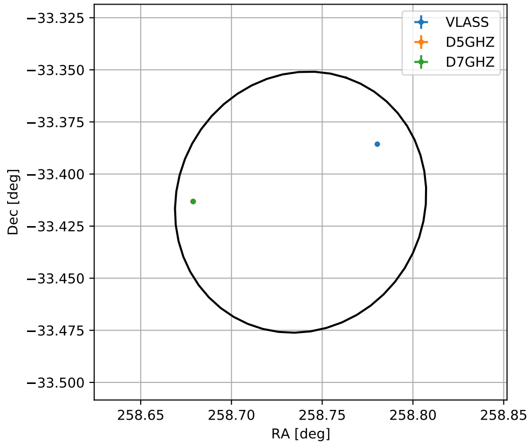
4FGL J1714.9-3324
