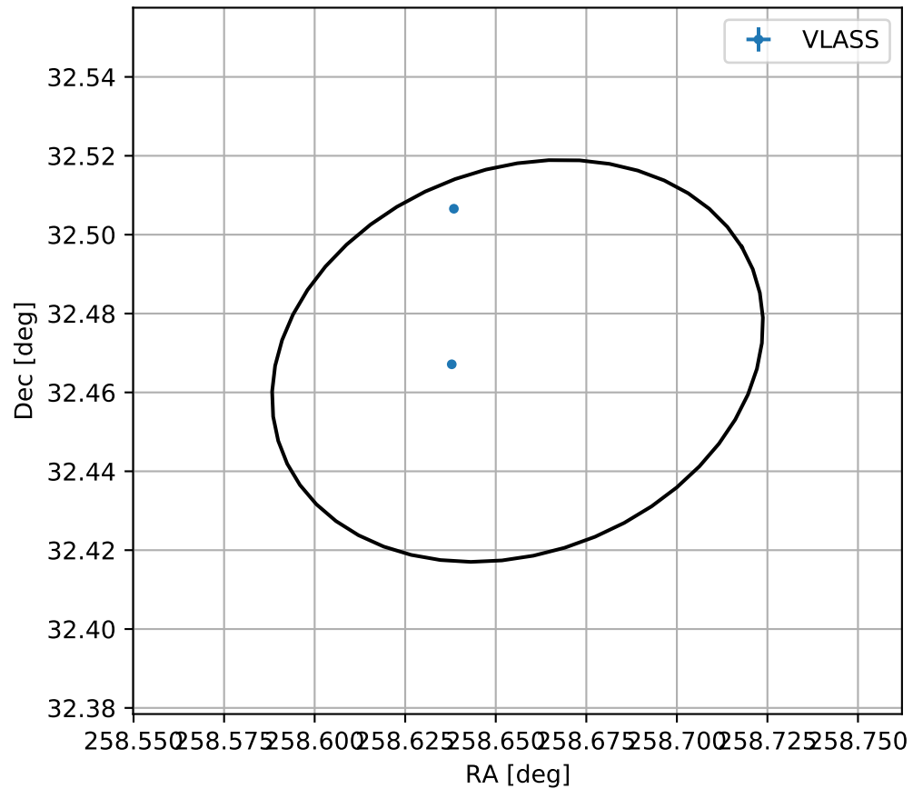
4FGL J1714.6+3228
