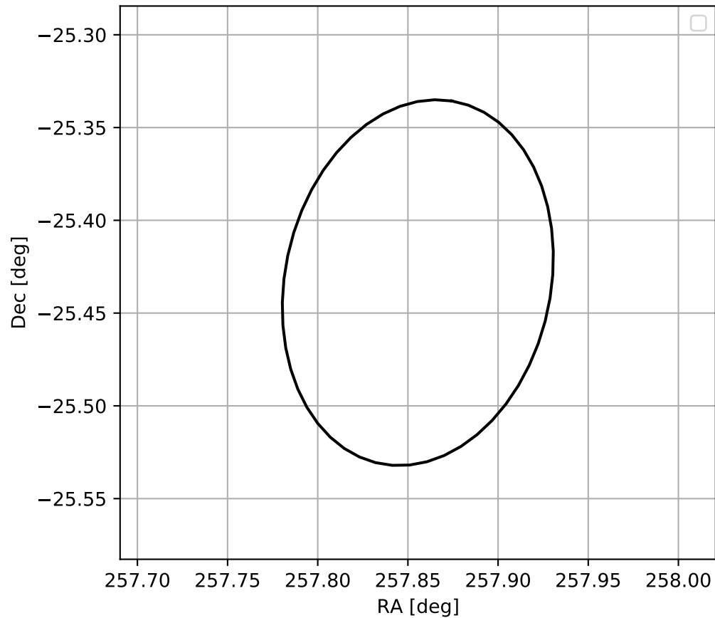
4FGL J1711.4-2526
