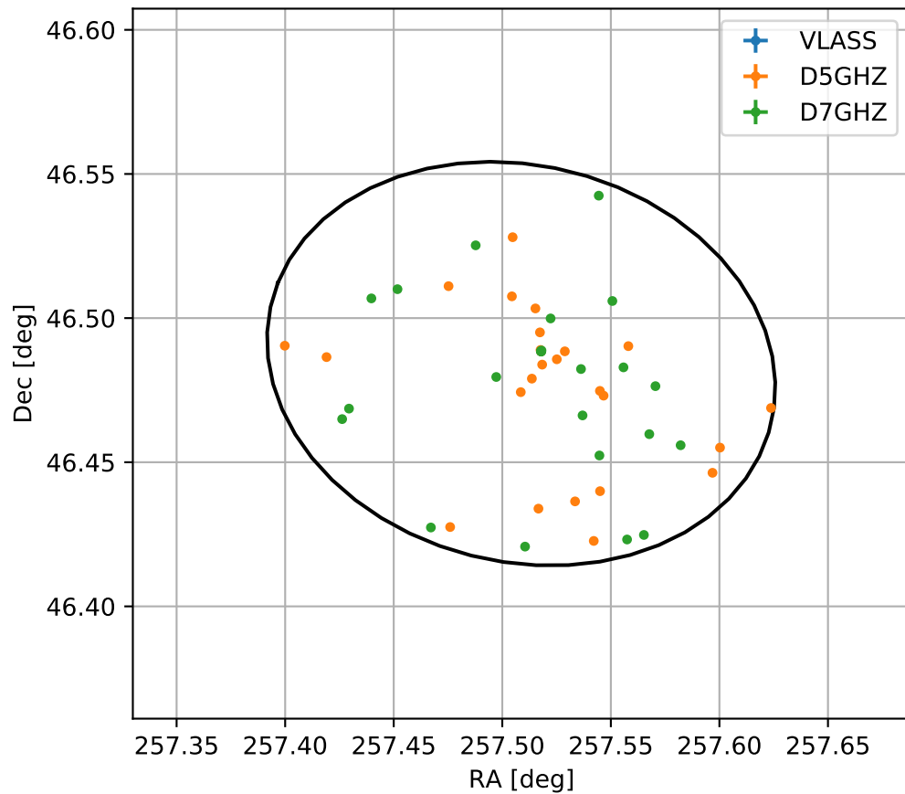
4FGL J1710.0+4629
