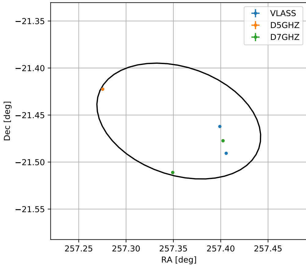
4FGL J1709.4-2127
