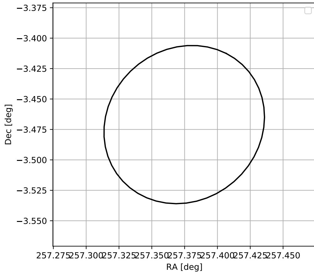
4FGL J1709.4-0328
