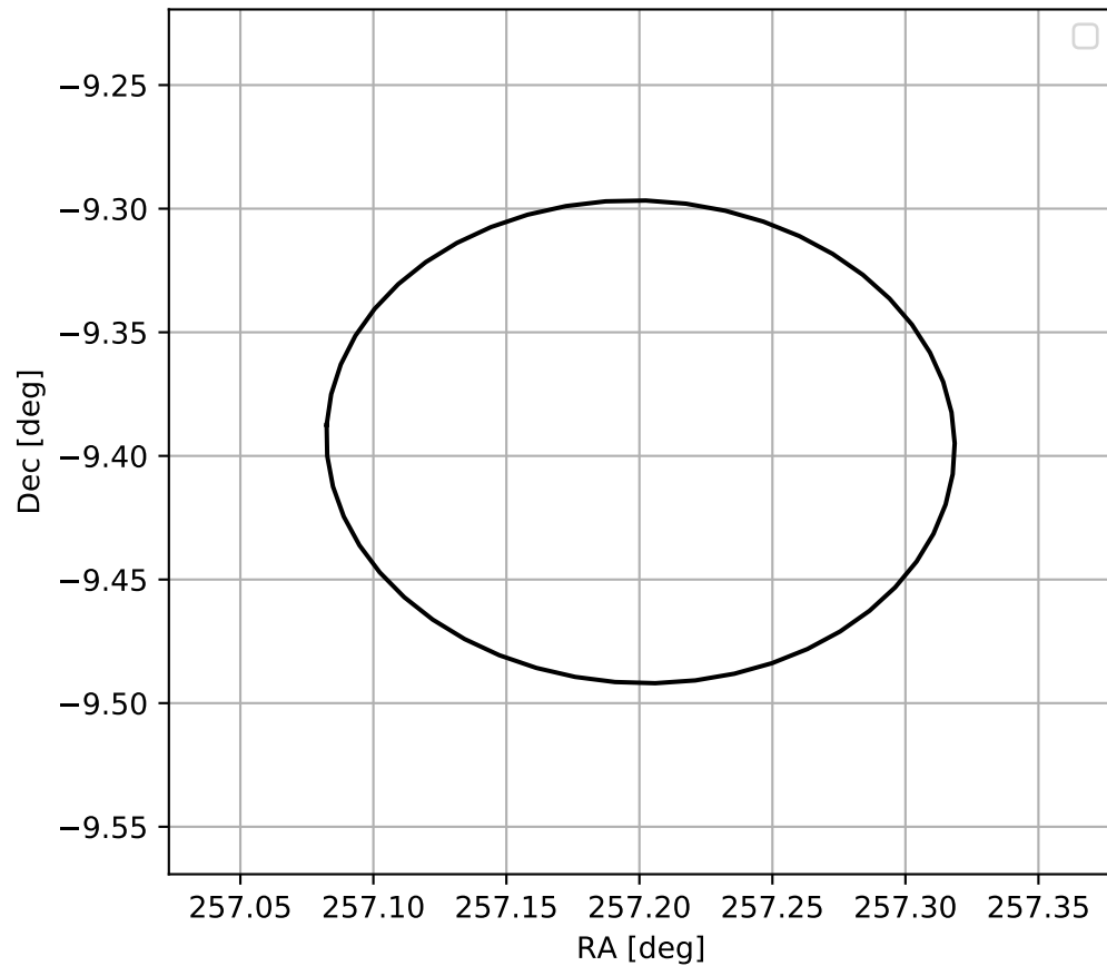
4FGL J1708.8-0923
