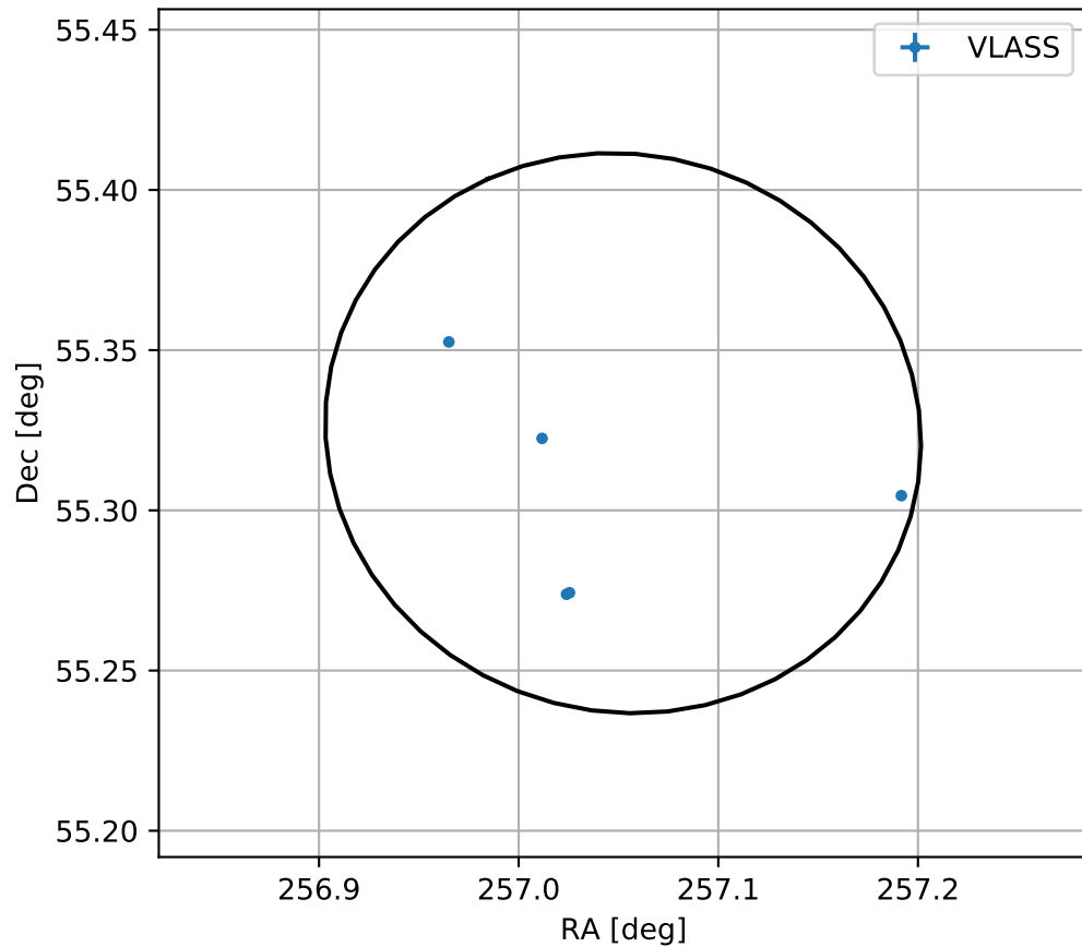
4FGL J1708.2+5519
