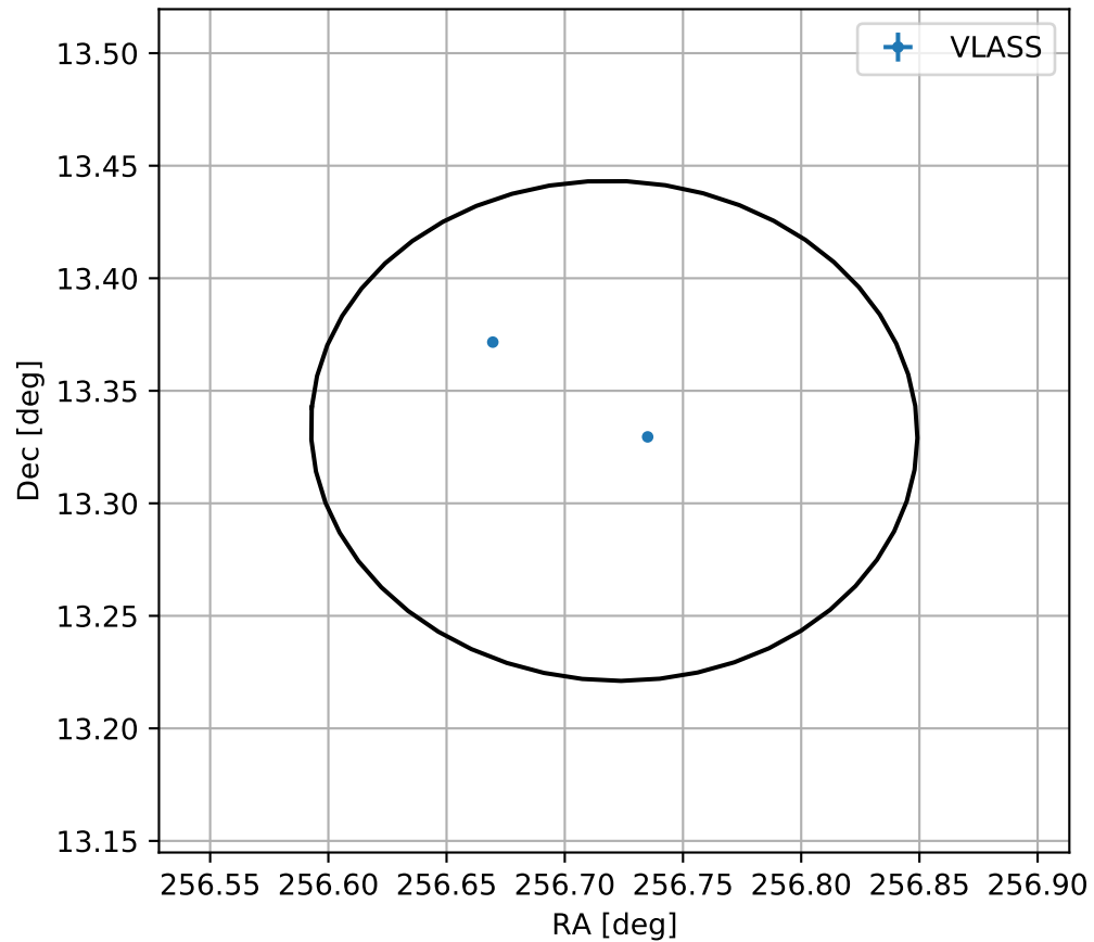
4FGL J1706.8+1319
