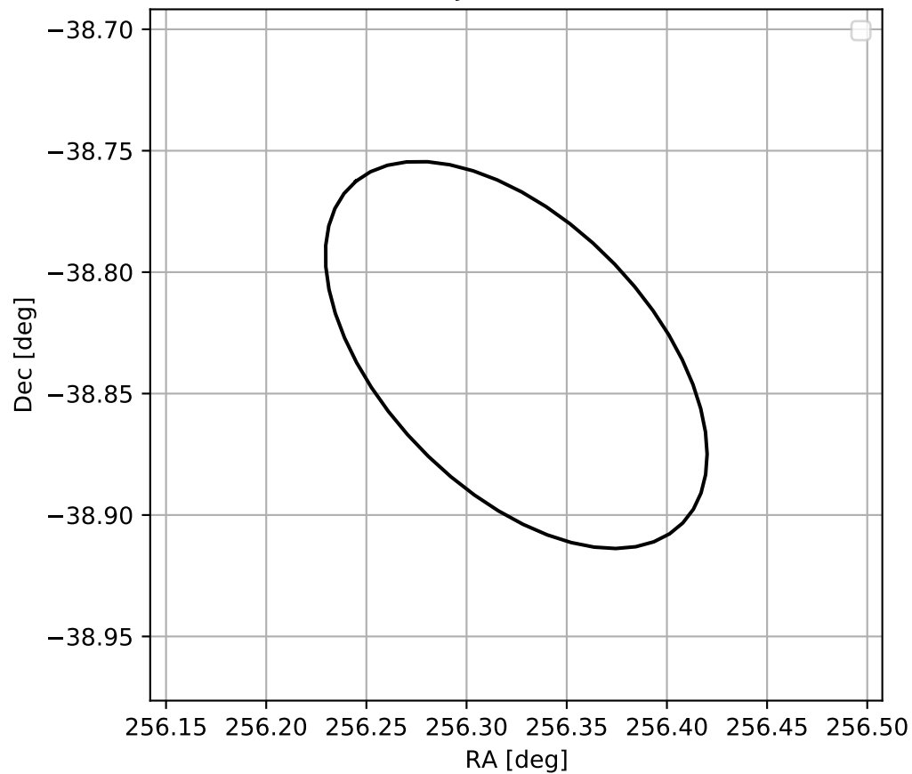
4FGL J1705.2-3850
