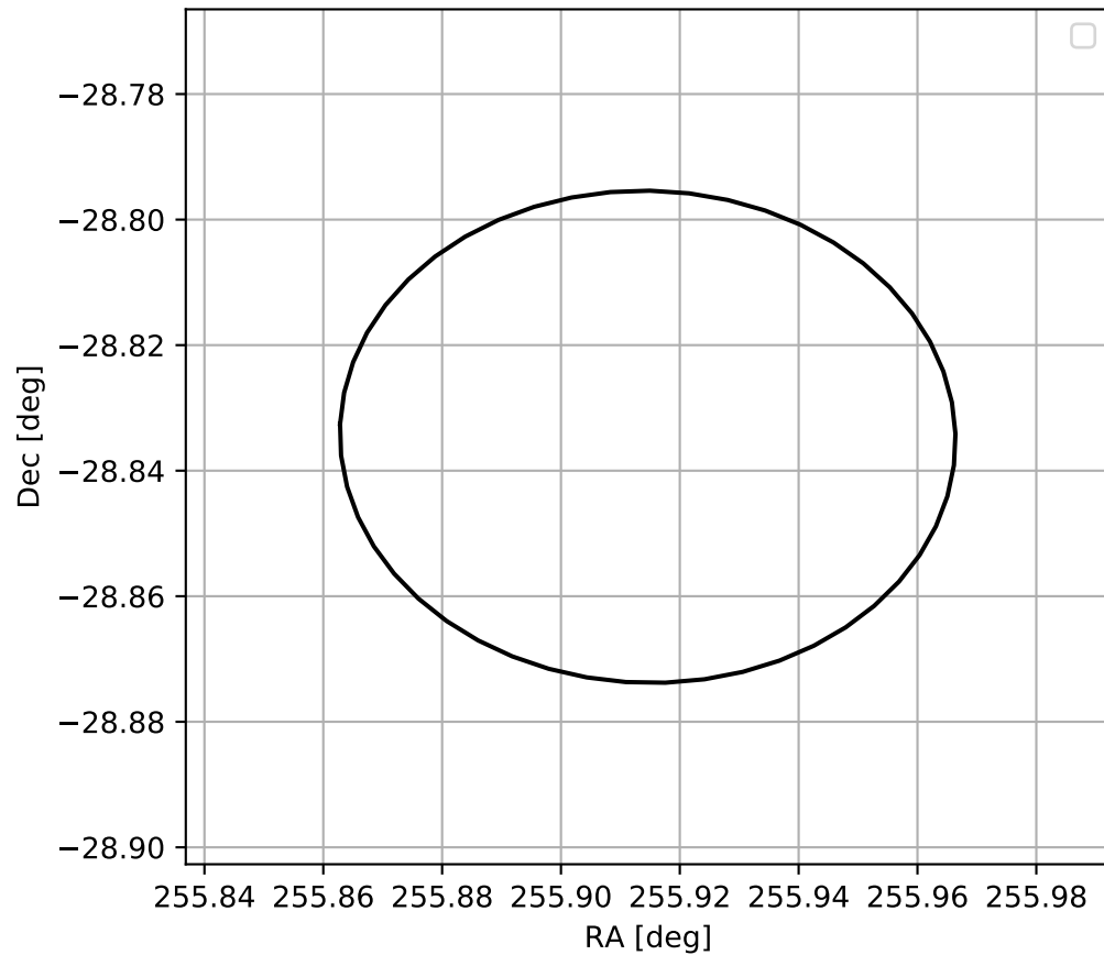
4FGL J1703.6-2850
