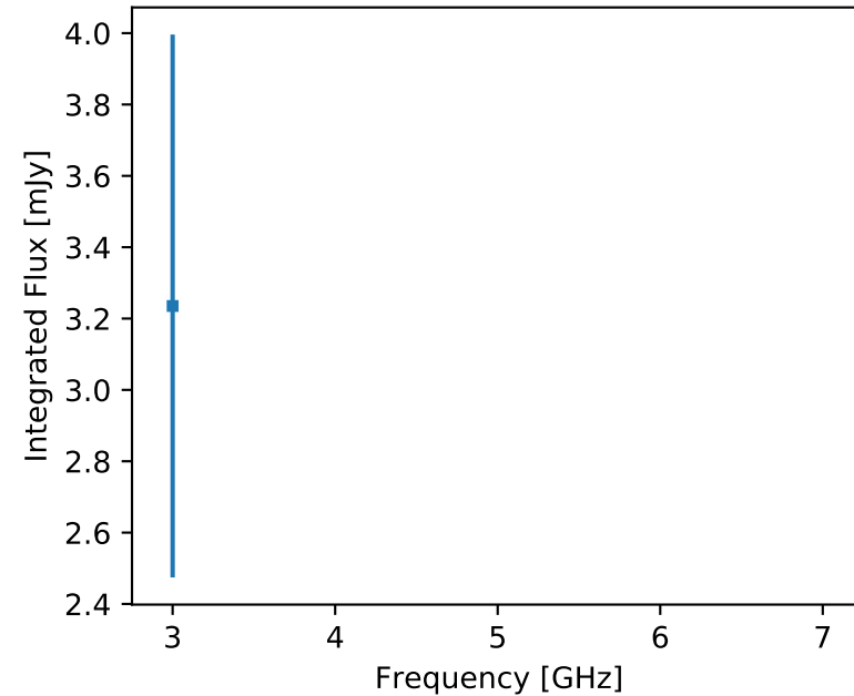
F357 J165831.58+431615.2 (unr)
