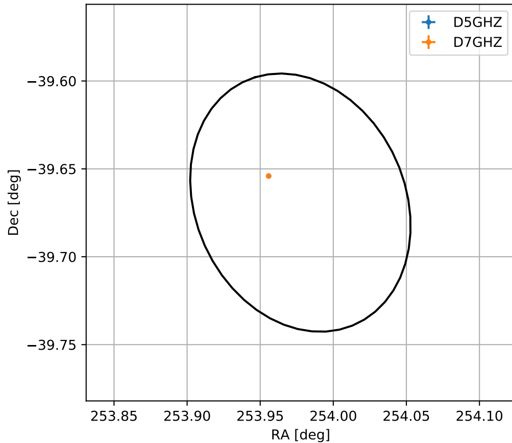
4FGL J1655.9-3940
