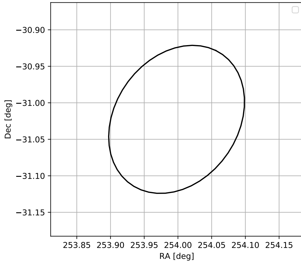
4FGL J1655.9-3101
