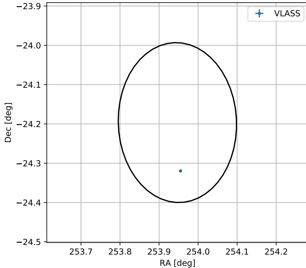
4FGL J1655.7-2411
