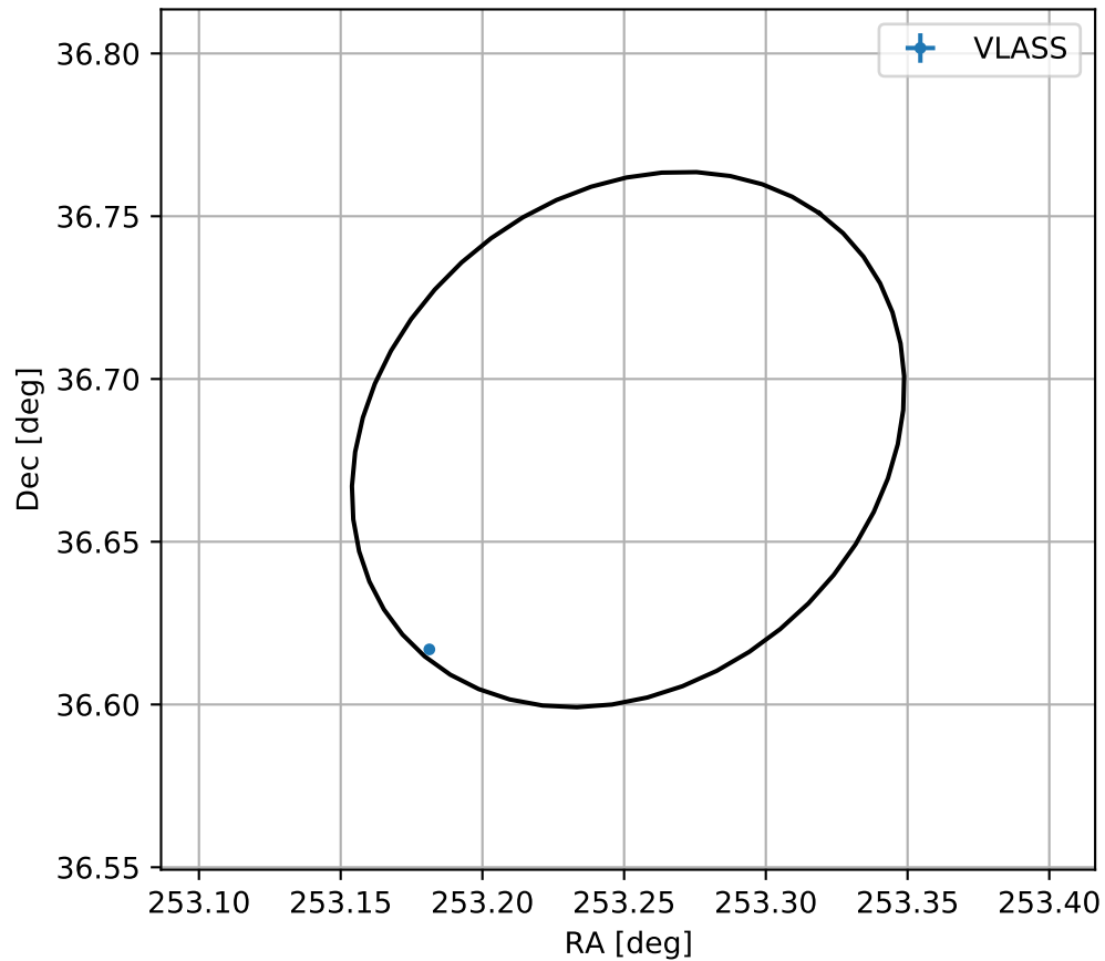
4FGL J1653.0+3640
