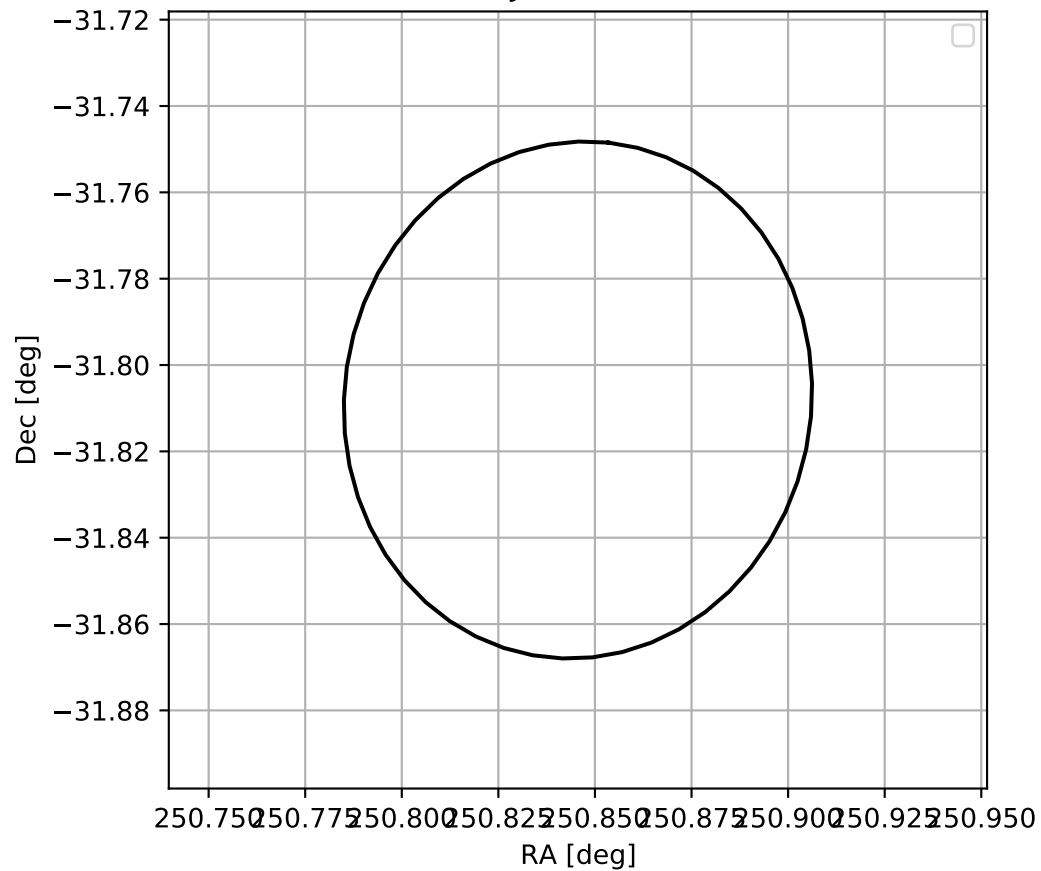
4FGL J1643.3-3148
