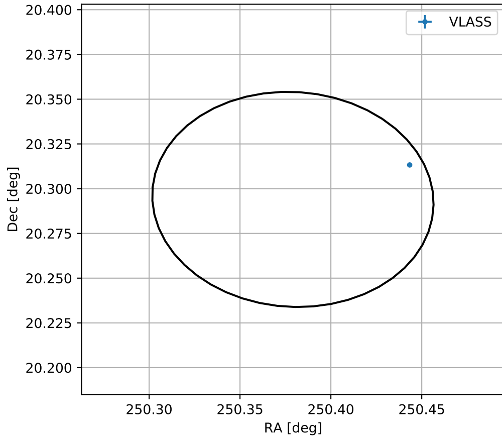
4FGL J1641.5+2017
