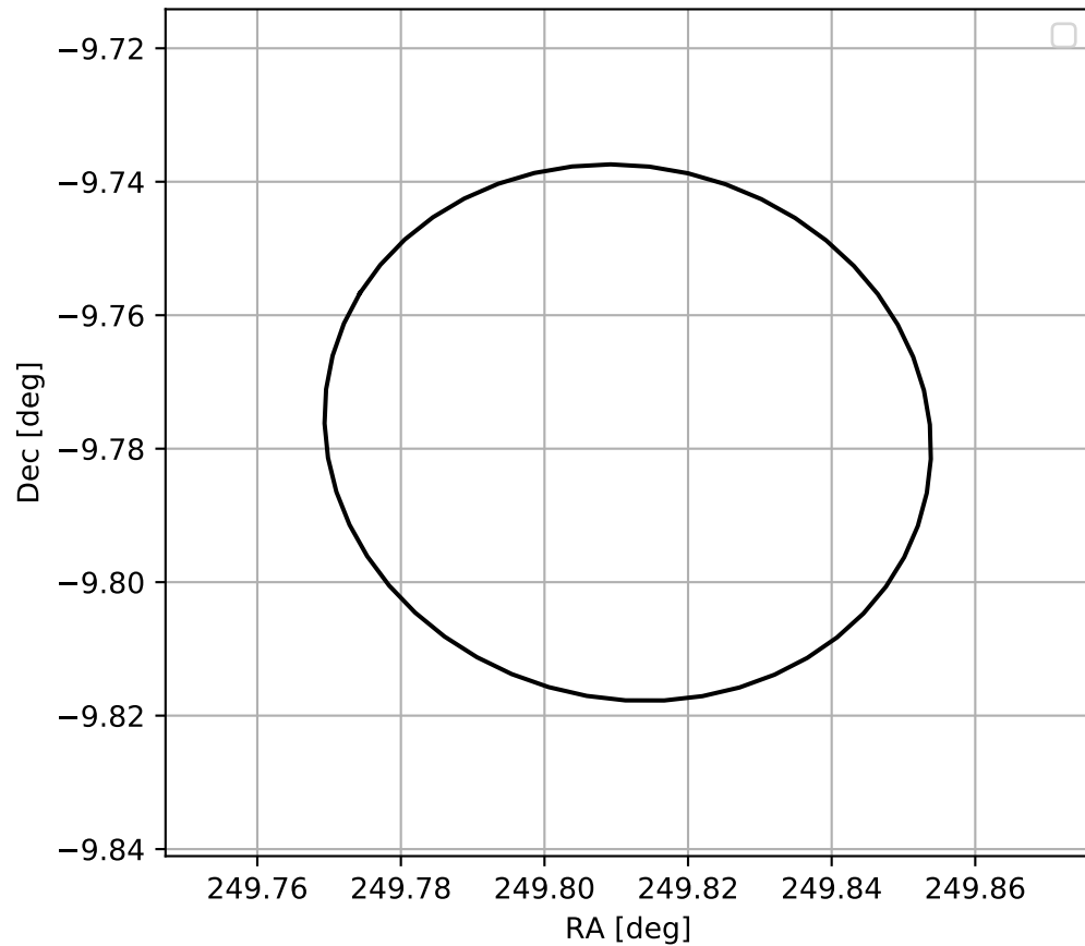
4FGL J1639.2-0946
