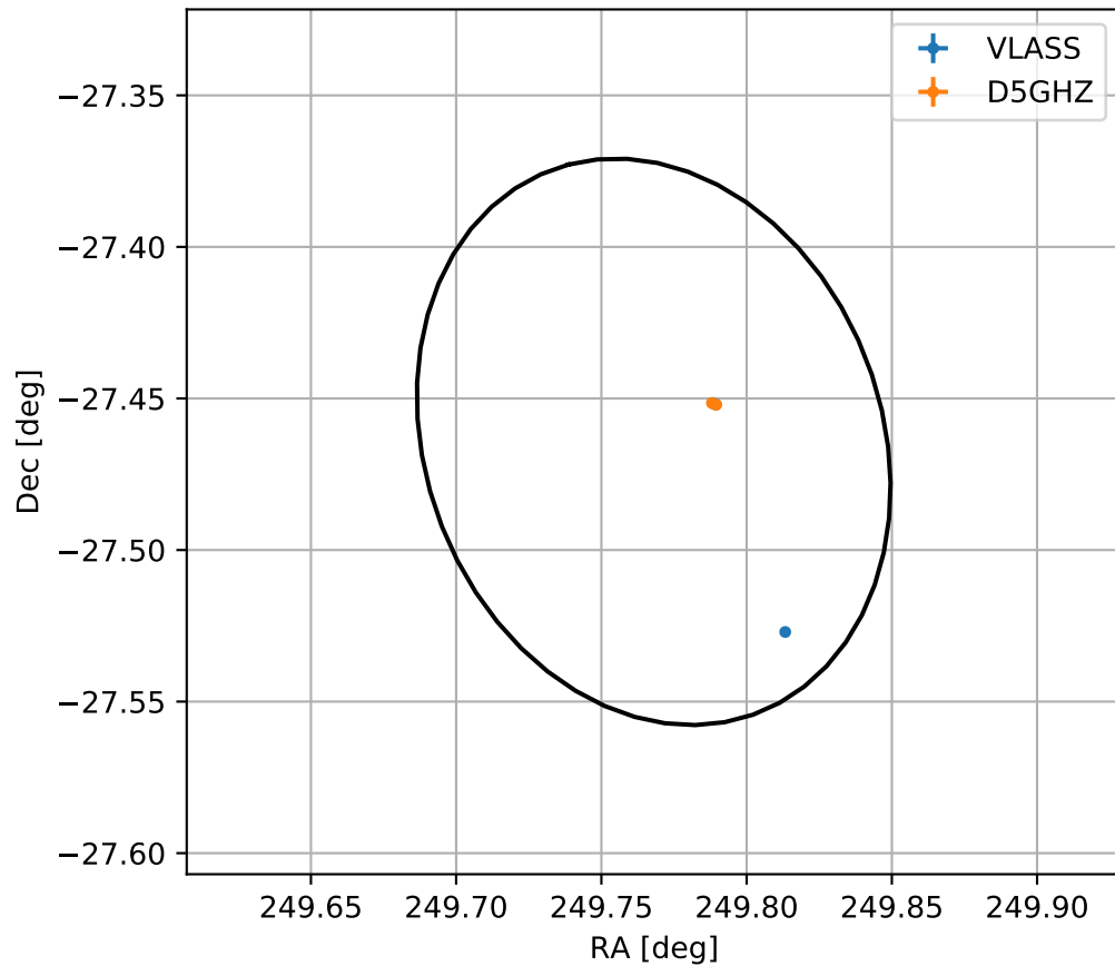
4FGL J1639.0-2727
