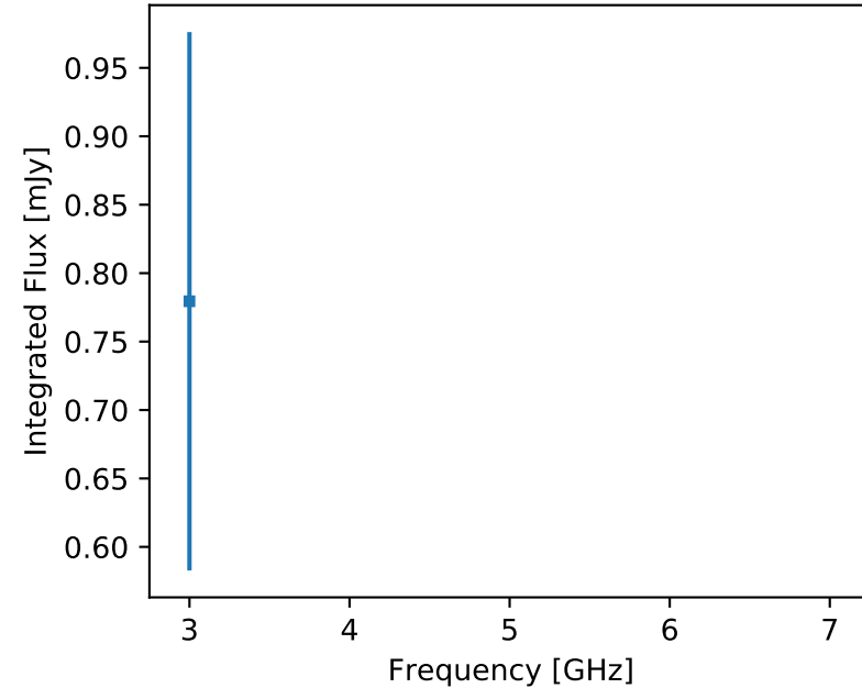
F357 J163146.72+414632.7 (unr)
