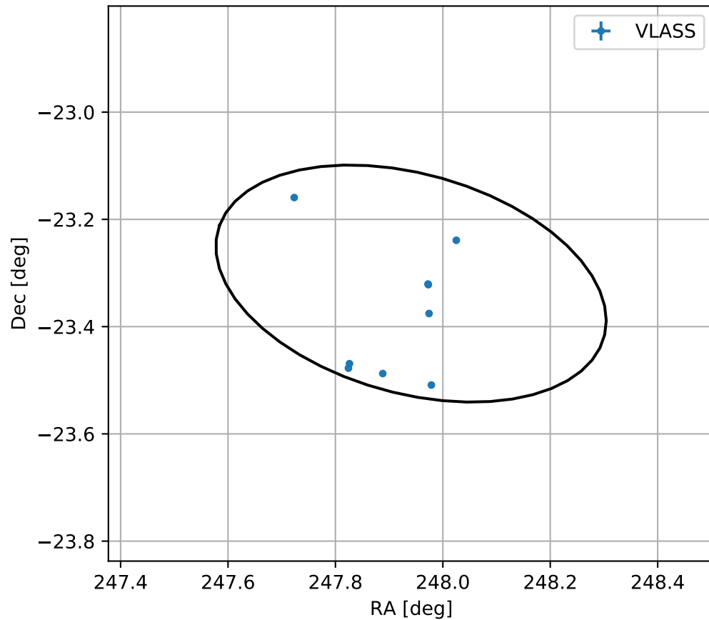
4FGL J1631.7-2319c
