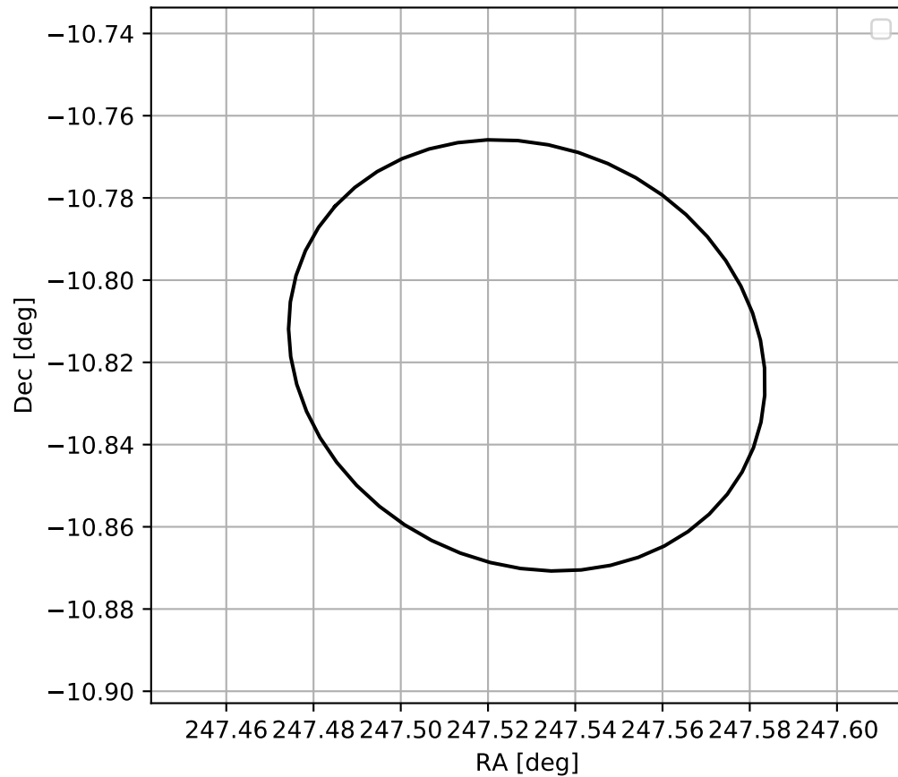
4FGL J1630.1-1049
