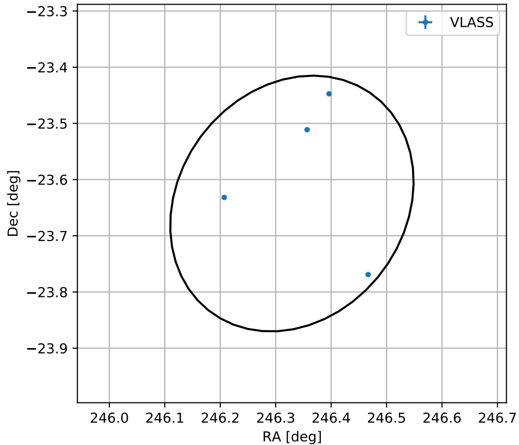
4FGL J1625.3-2338c
