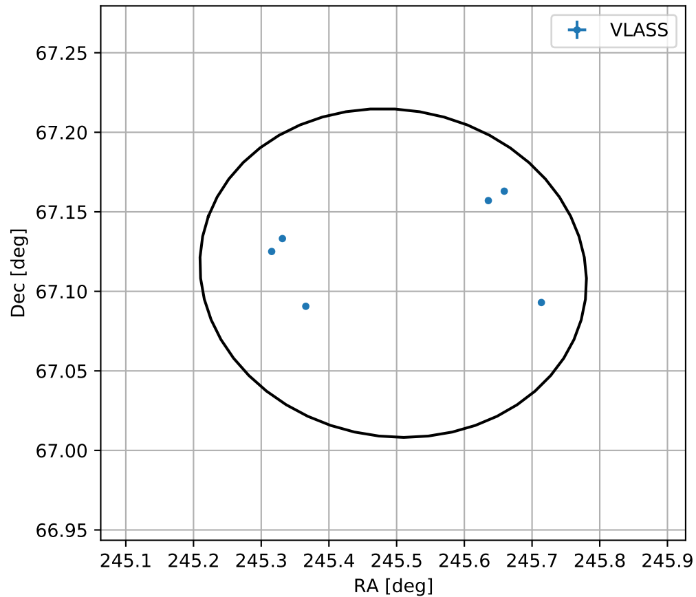
4FGL J1621.9+6706
