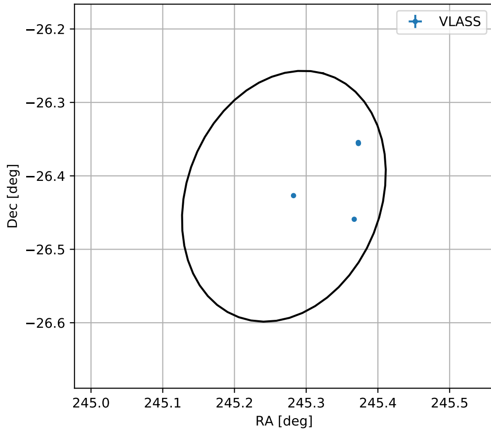
4FGL J1621.0-2625
