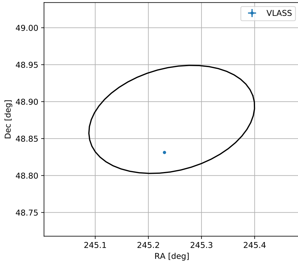
4FGL J1620.9+4852
