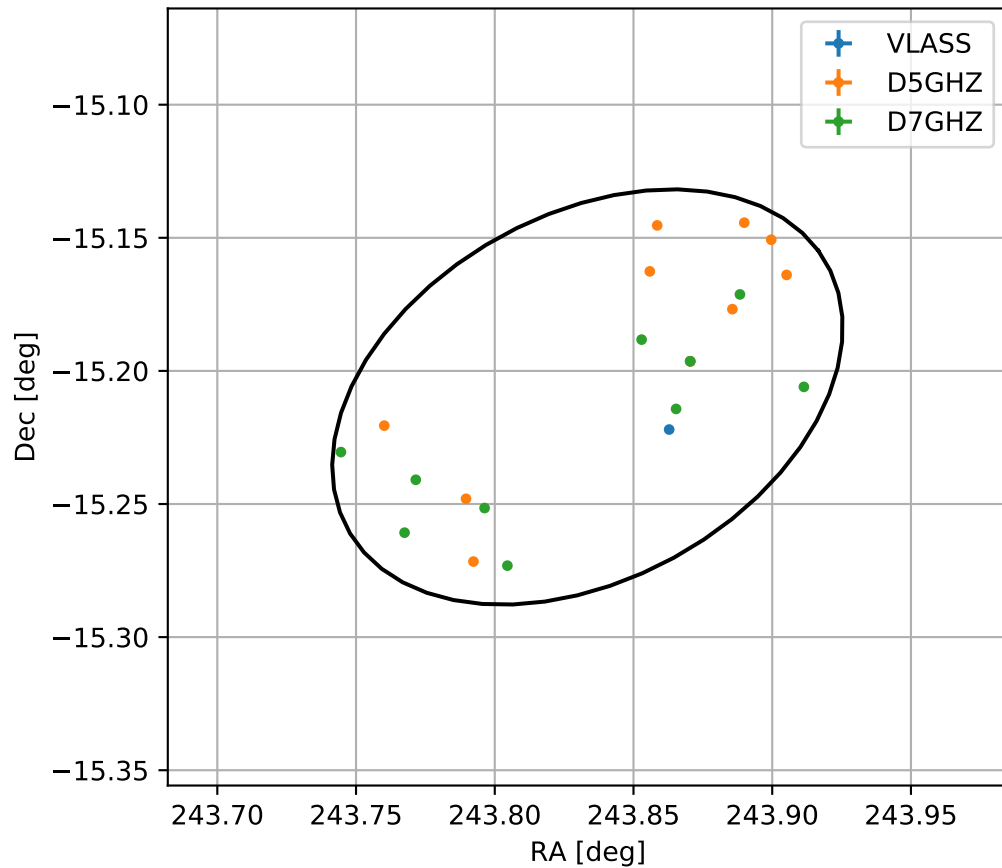
4FGL J1615.3-1512
