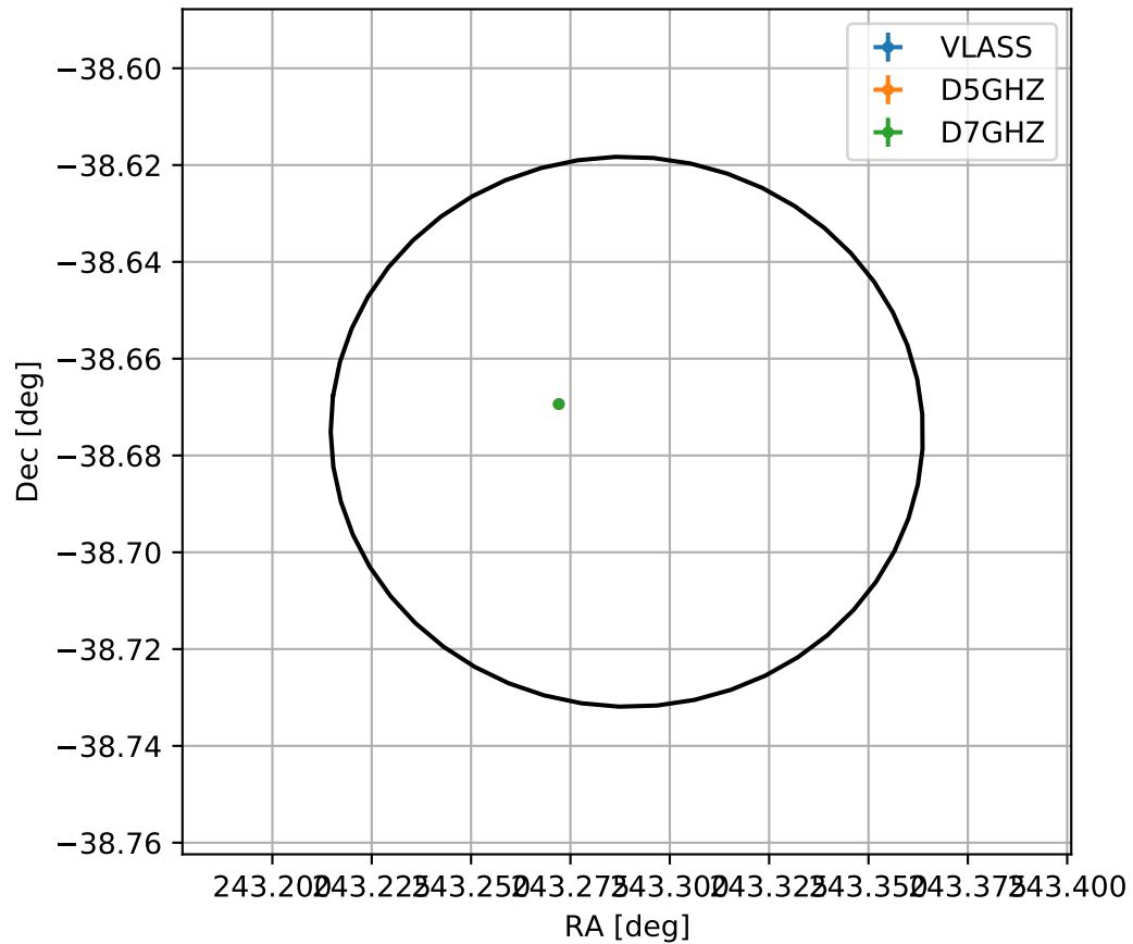
4FGL J1613.1-3840
