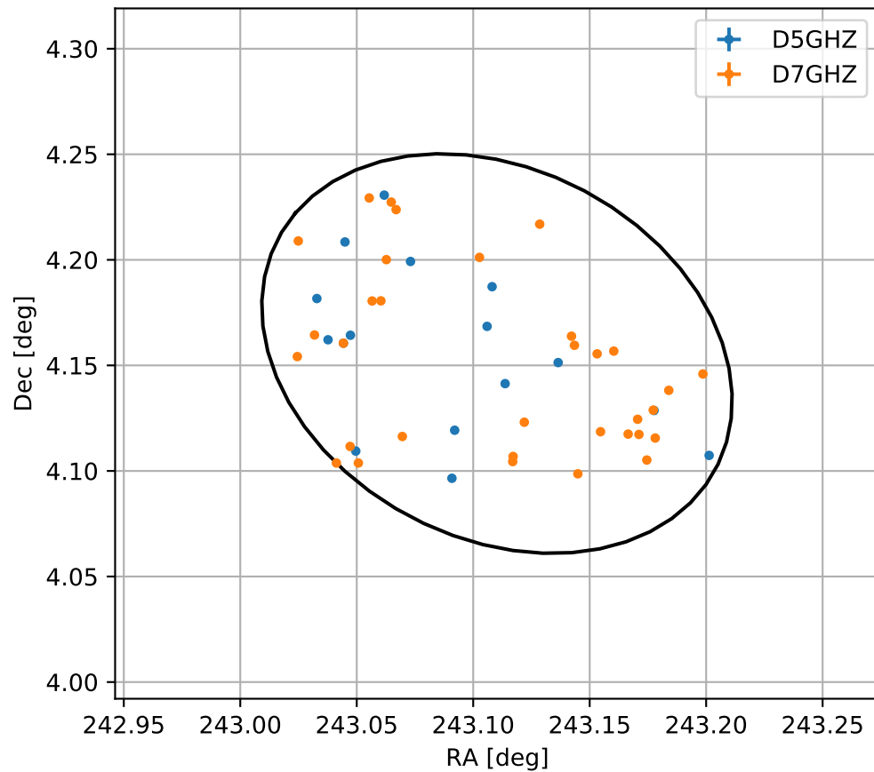
4FGL J1612.4+0409
