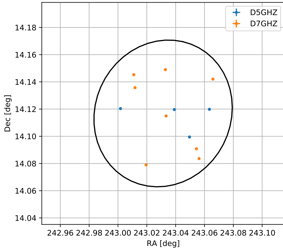
4FGL J1612.1+1407
