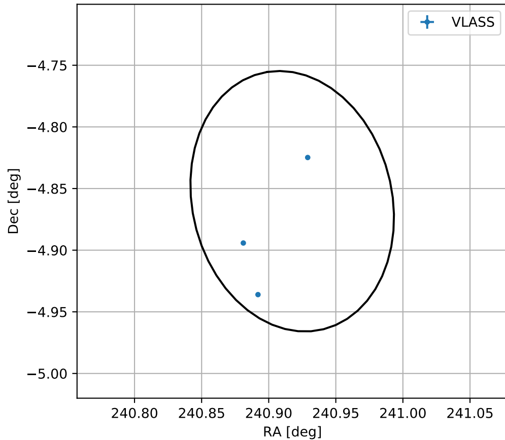
4FGL J1603.6-0451
