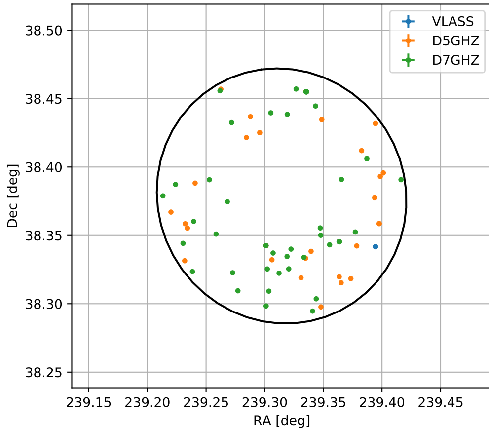
4FGL J1557.2+3822
