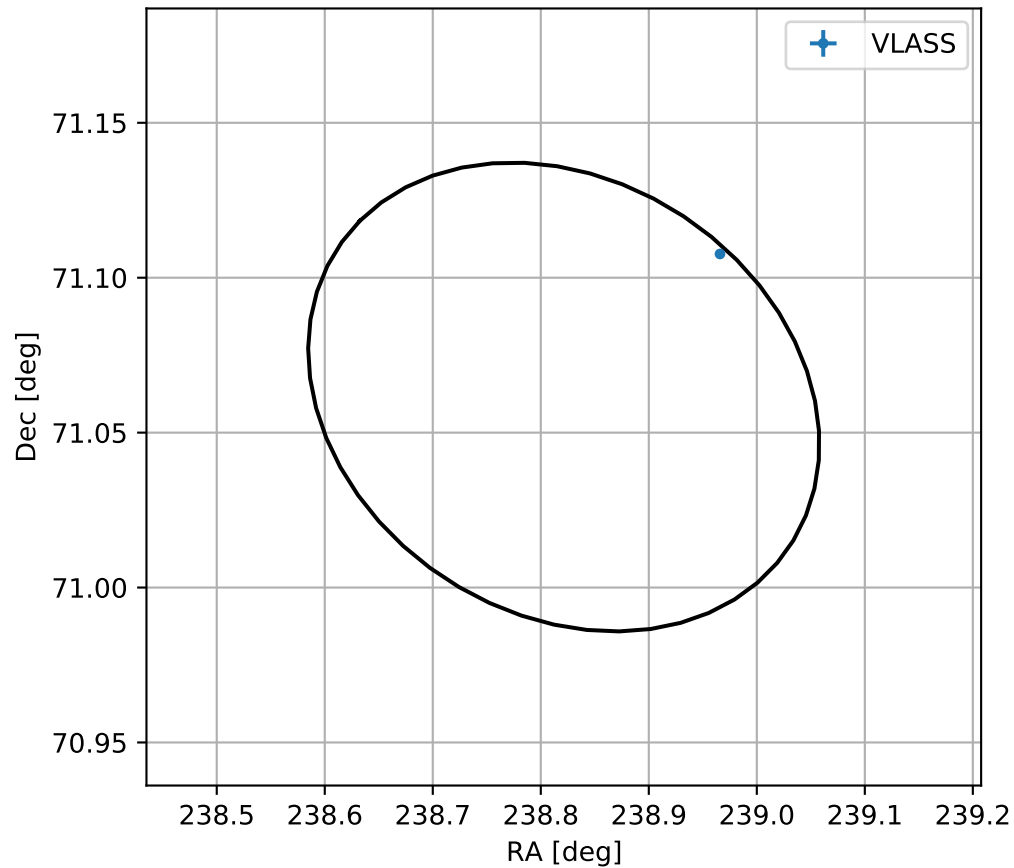
4FGL J1555.2+7103
