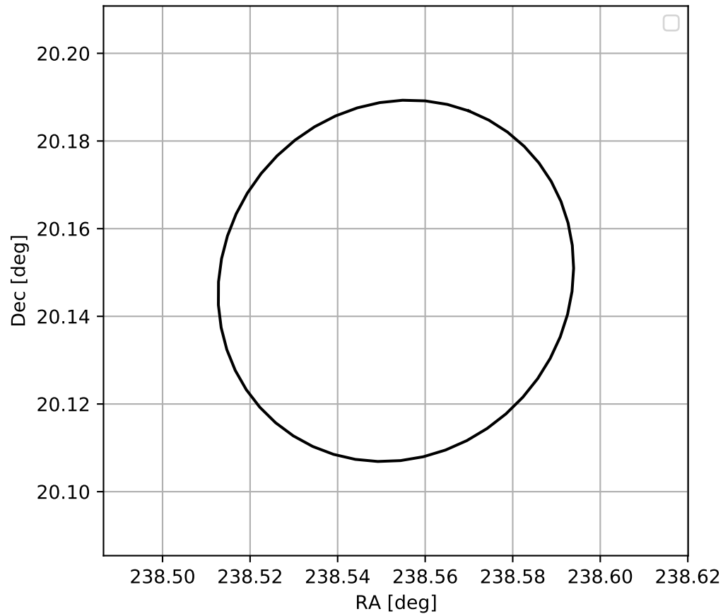
4FGL J1554.2+2008
