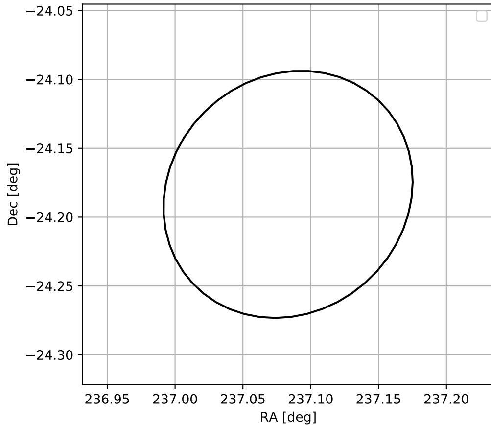
4FGL J1548.3-2411
