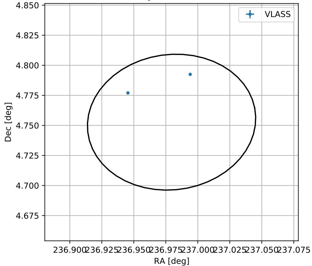
4FGL J1547.9+0445
