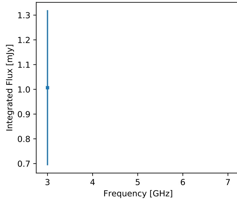
F357 J154758.57+044732.8 (unr)
