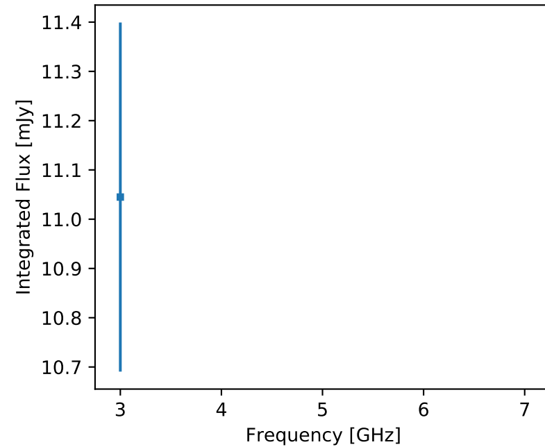
F357 J154758.57+044732.8 (unr)
