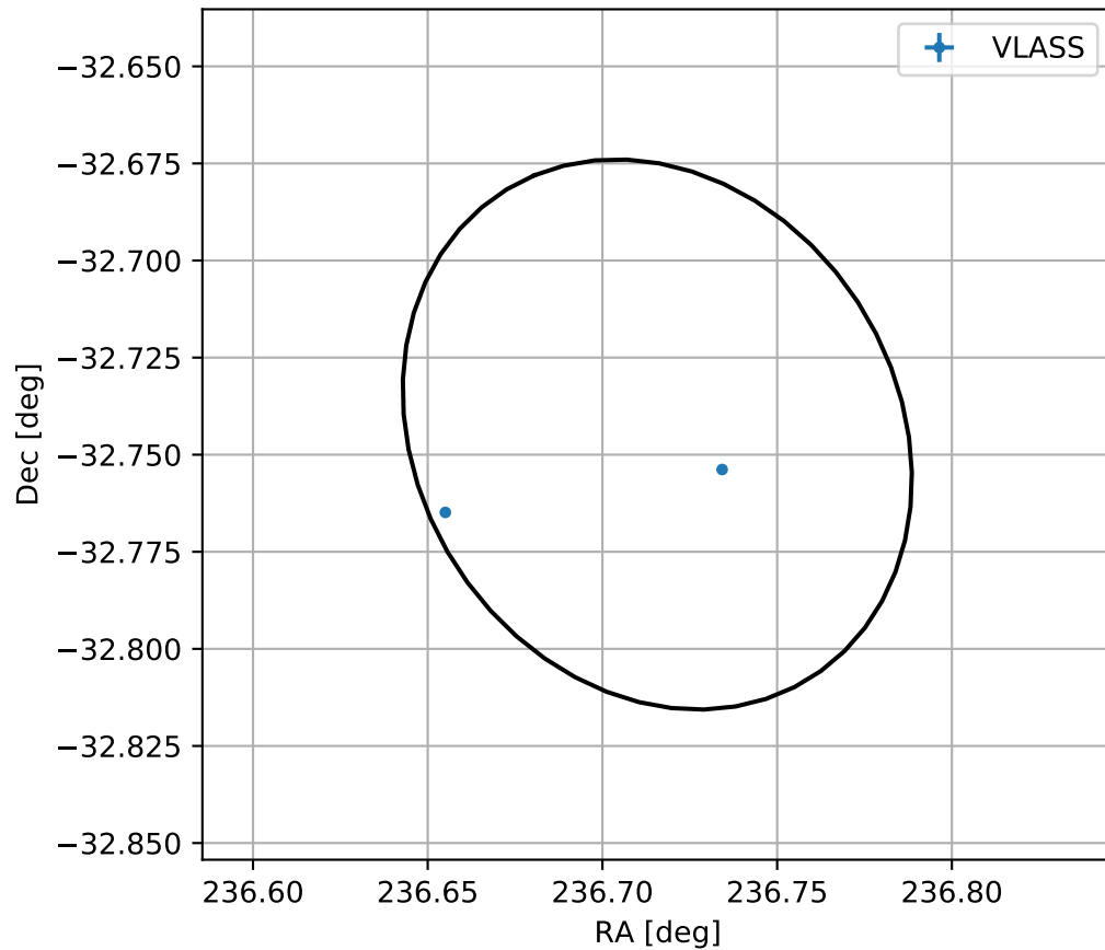
4FGL J1546.8-3244
