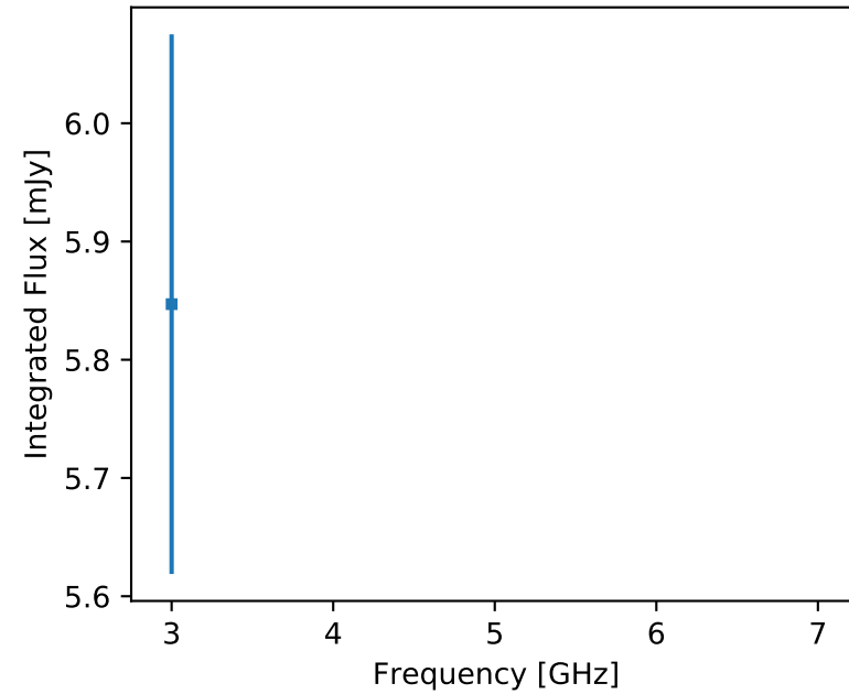
F357 J154550.30+284102.3 (unr)
