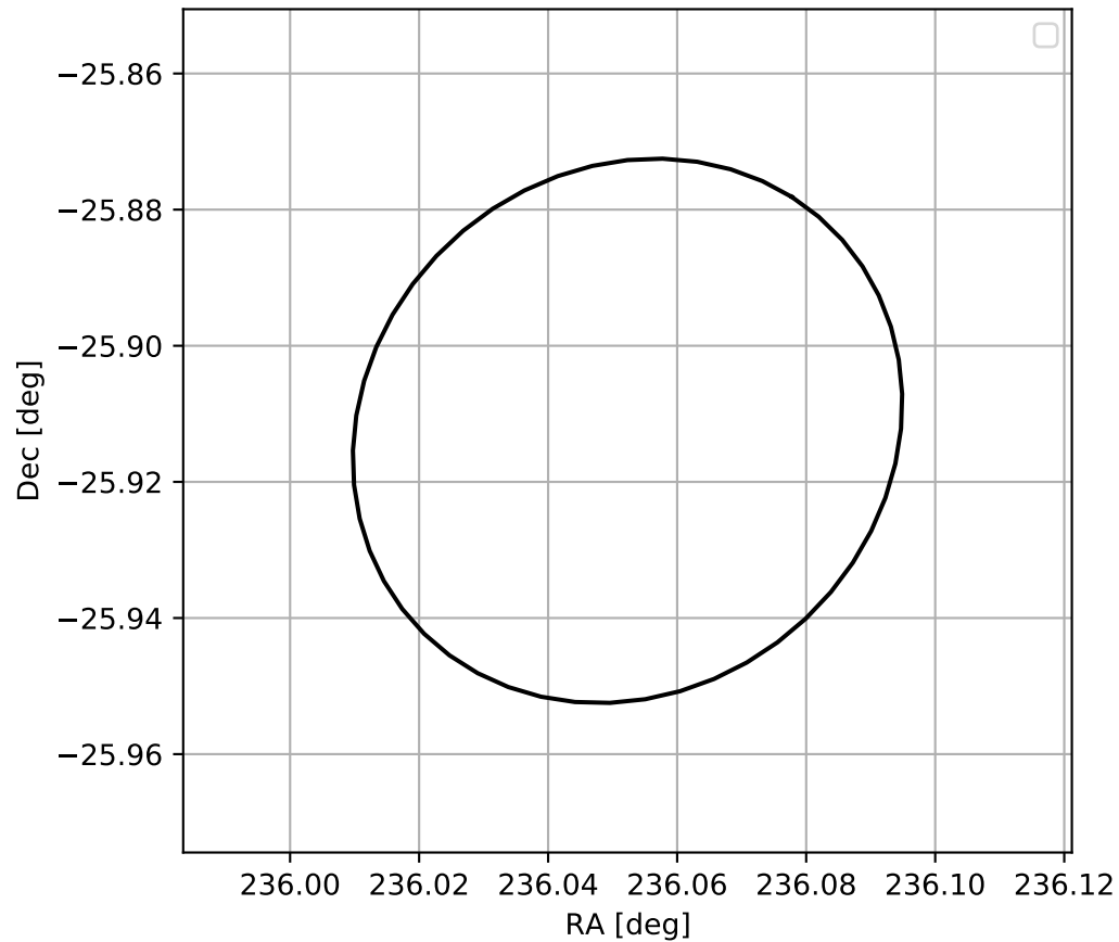
4FGL J1544.2-2554
