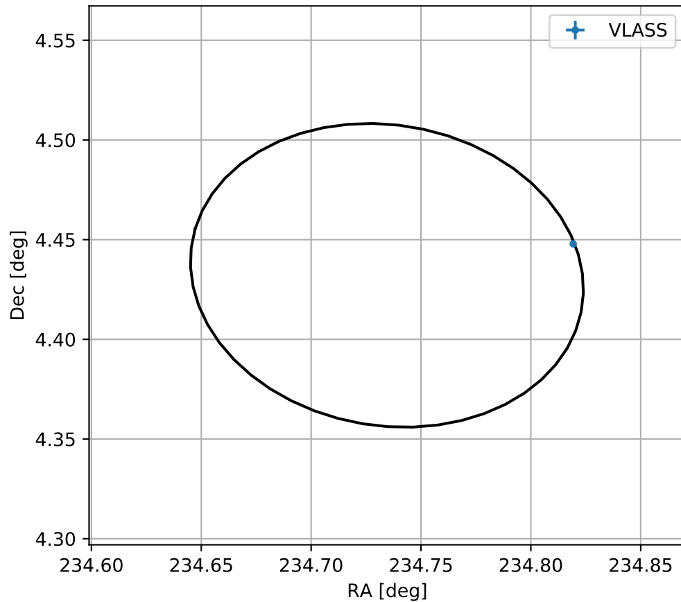
4FGL J1538.9+0425
