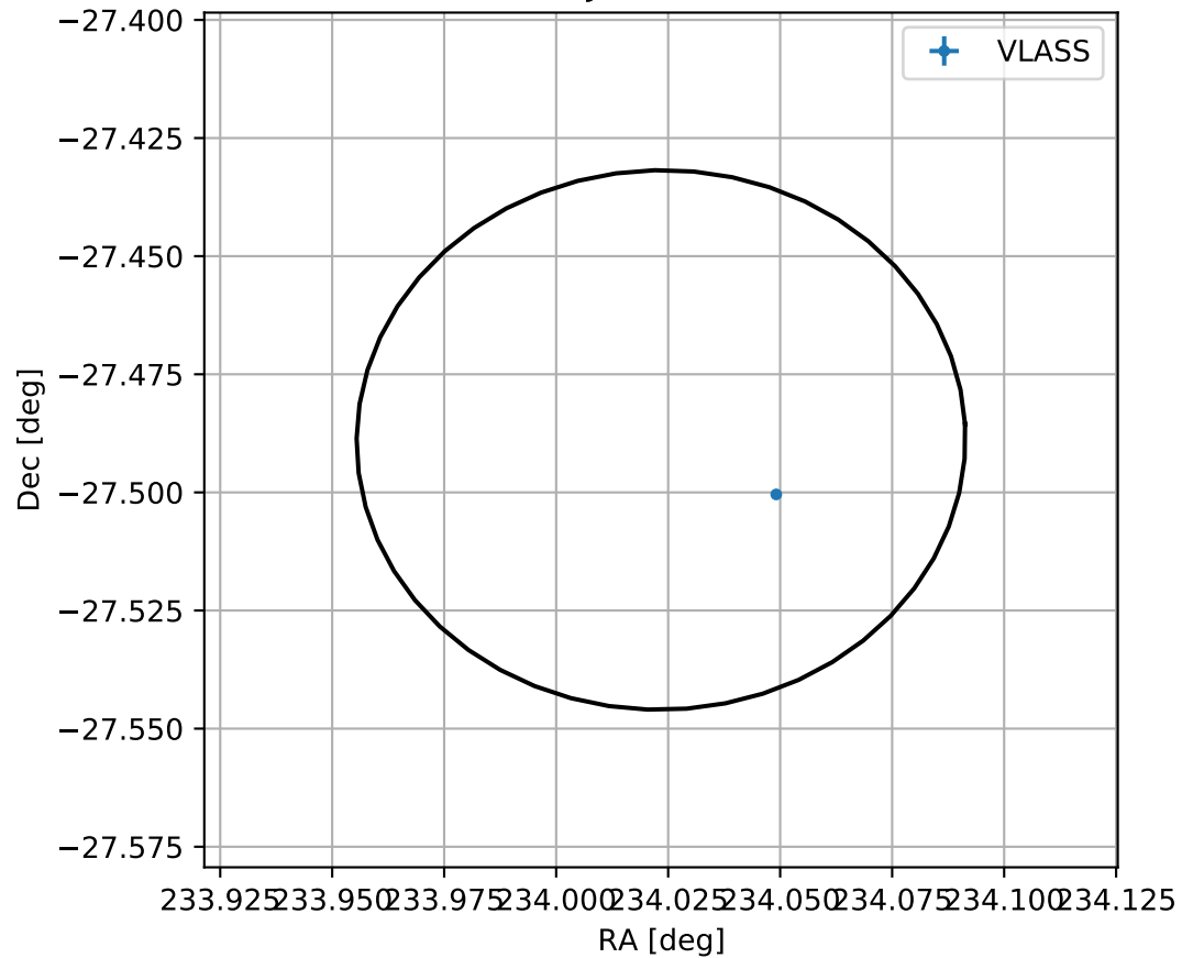
4FGL J1536.0-2729
