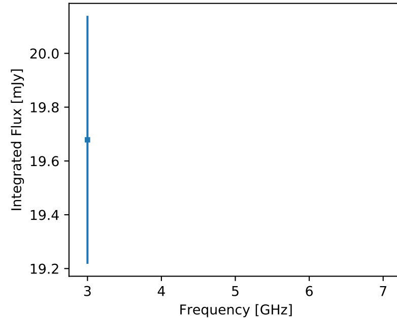
F357 J153611.79-273001.5 (unr)
