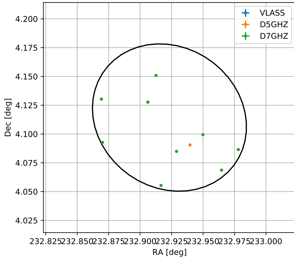
4FGL J1531.6+0406
