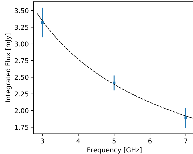
F357 J152835.77+200420.1 (unr)
